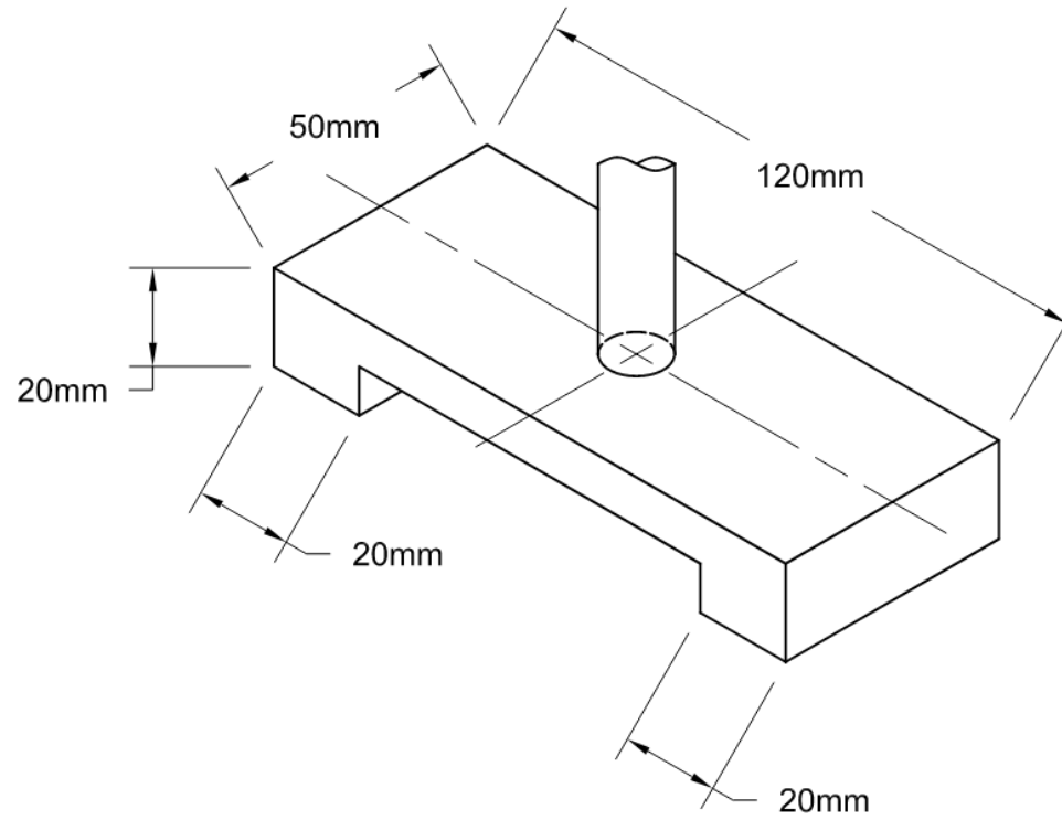
FIGURE 4 LOADING DEVICE (NOT TO SCALE)
